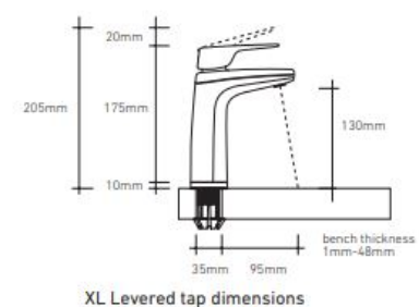
XL Levered tap dimensions
